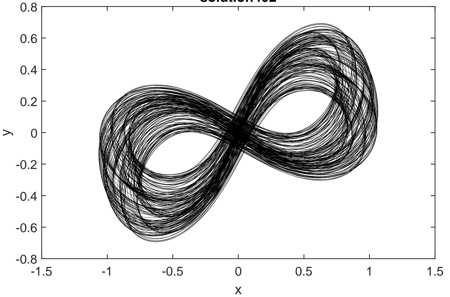
solution402
