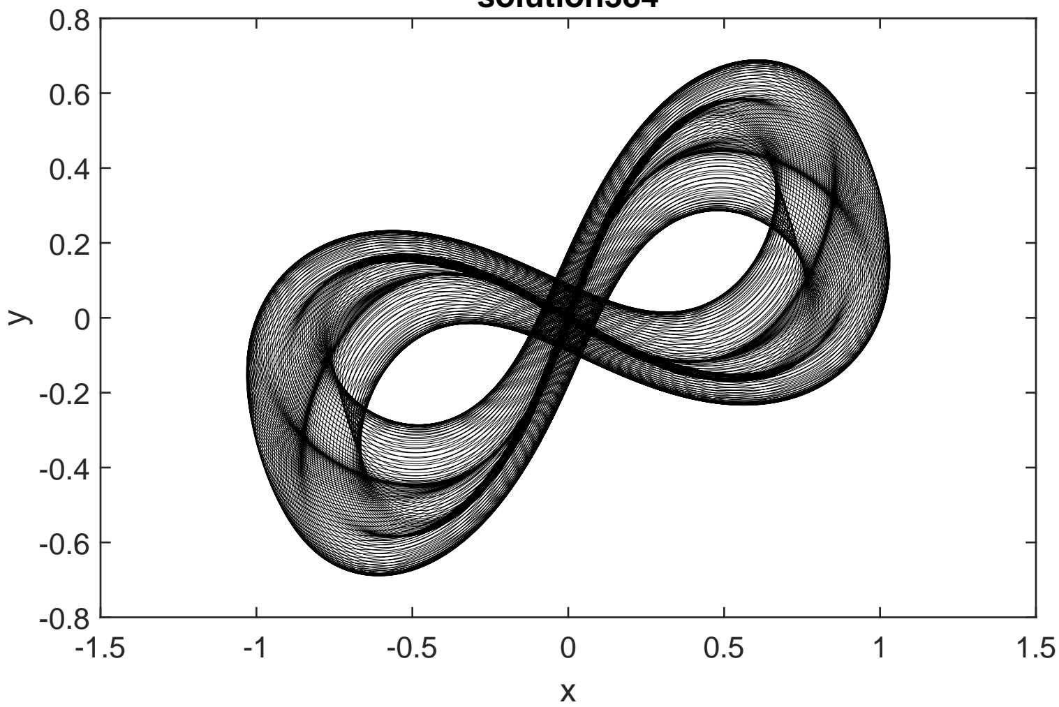
solution384
