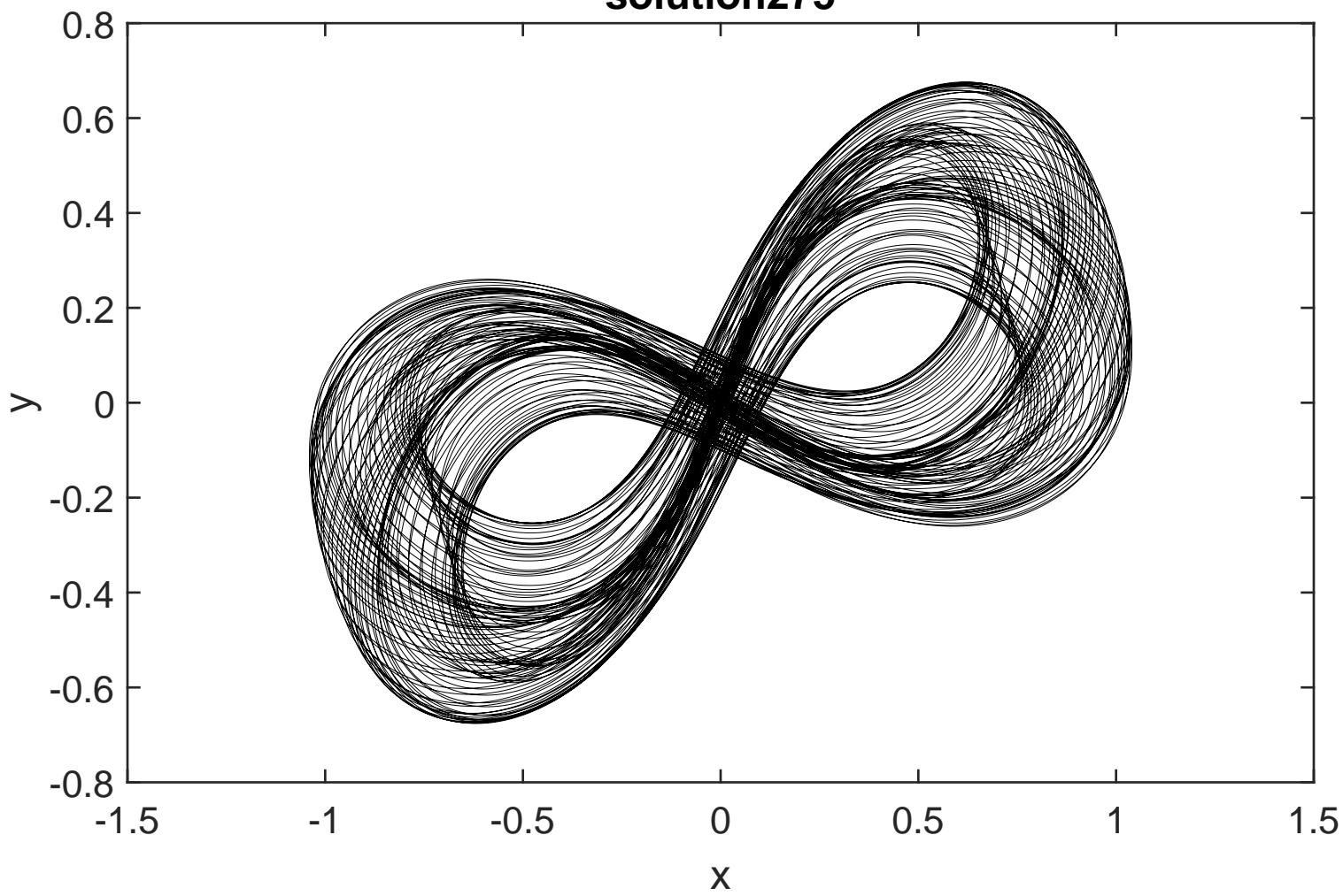
solution275
