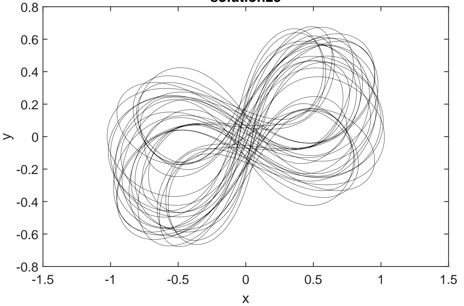
solution23
