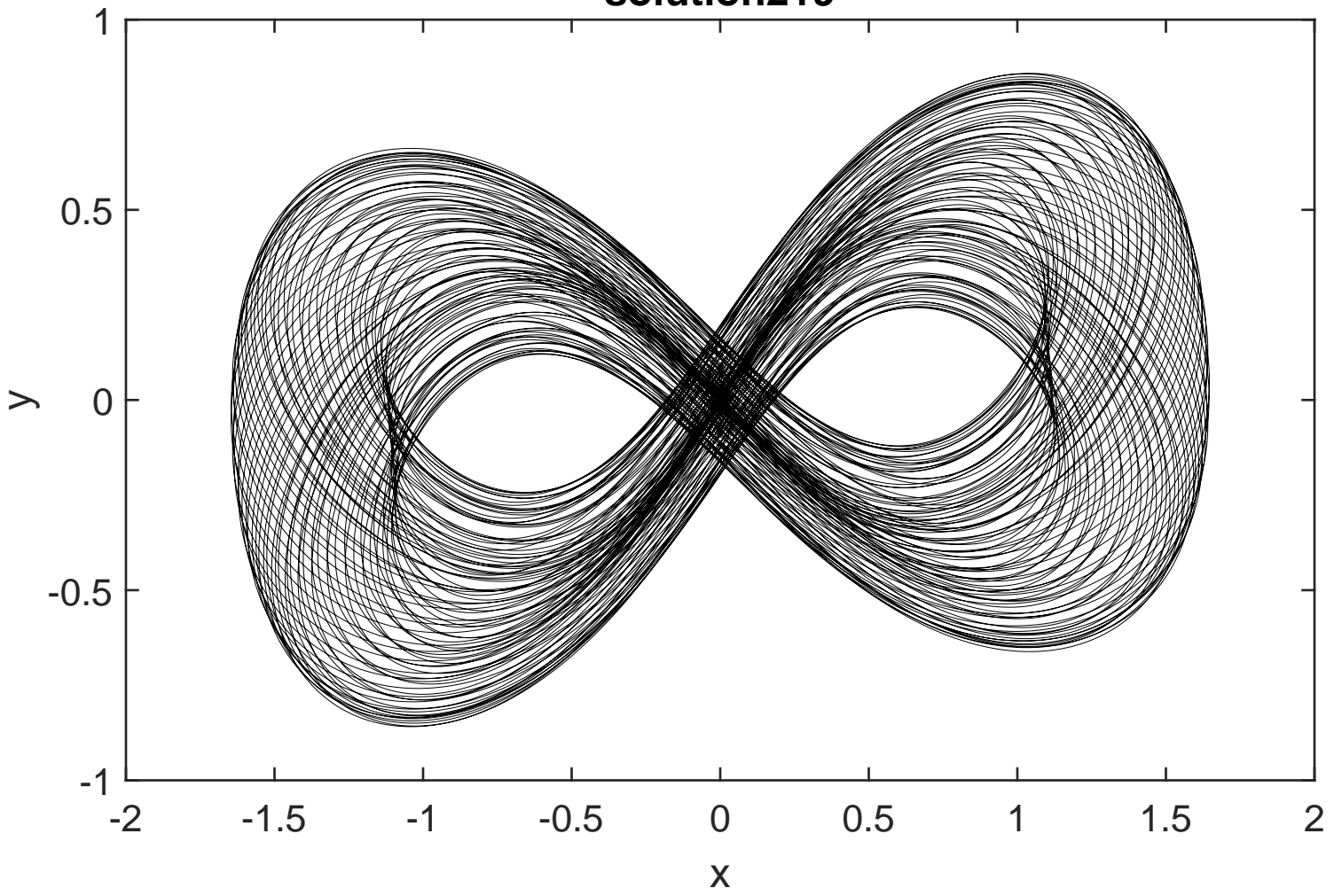
solution219
